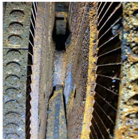
Rotor Blading, Typical
