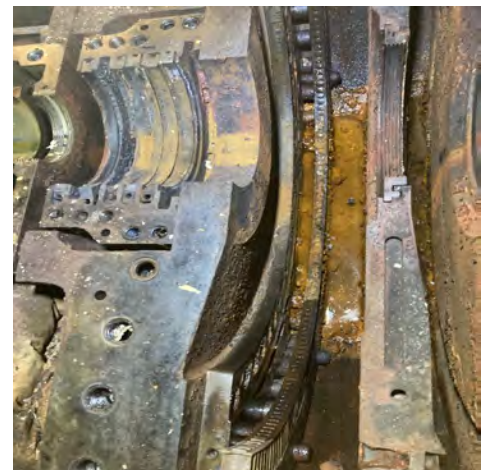
Reversing Segments Prior to Removal
