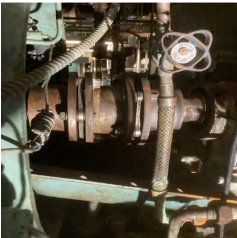
Coupling Assembly As Found Prior to Disassembly
