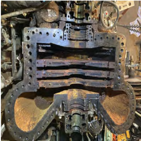
Lower Casing with Diaphragms as Found
