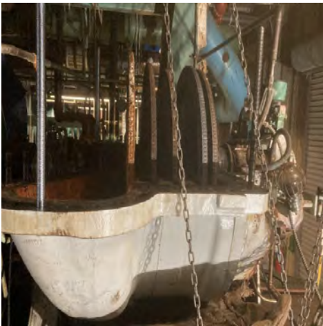
Upper Casing Removed, Rotor at Splitline
