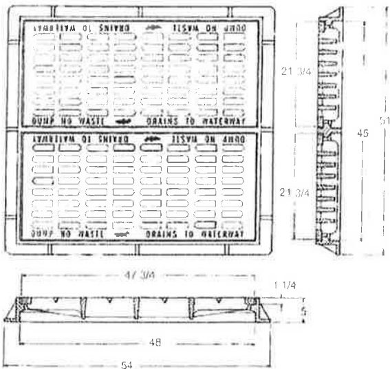
BICYCLE-SAFE GRATE
