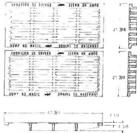
ALTERNATE STREAM FLOW GRATES NOT RECOMMENDED FOR BICYCLE TRAFFIC
