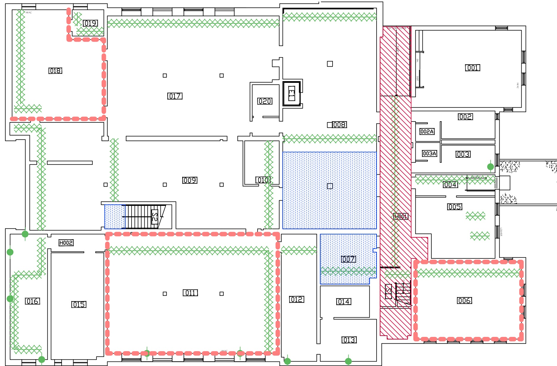
BASEMENT PLAN SCALE: 1/16" = 1' - 0"
