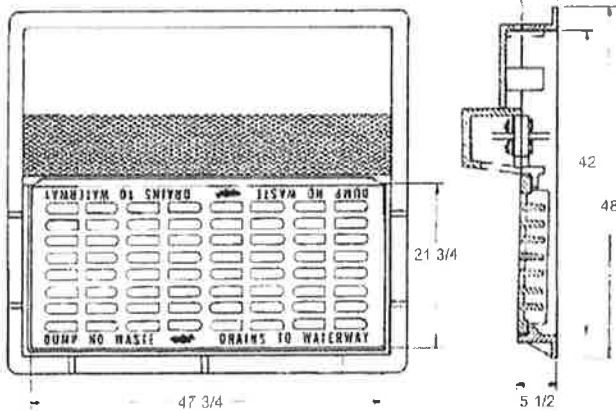
TYPE 'B' INLET WITH BICYCLE-SAFE GRATE
