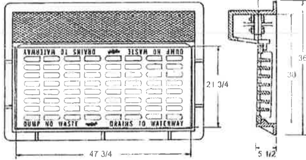
TYPE 'D' INLET WITH BICYCLE-SAFE GRATE
