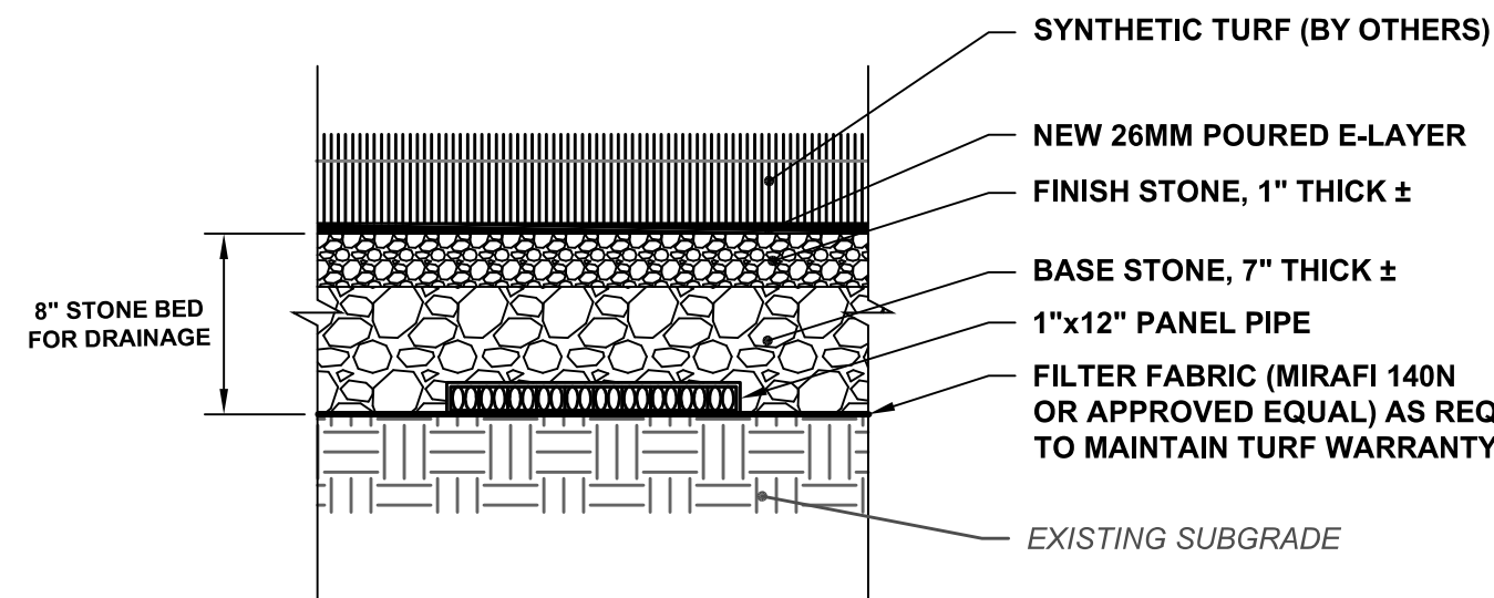
E-LAYER AND BASE DETAIL N.T.S.
