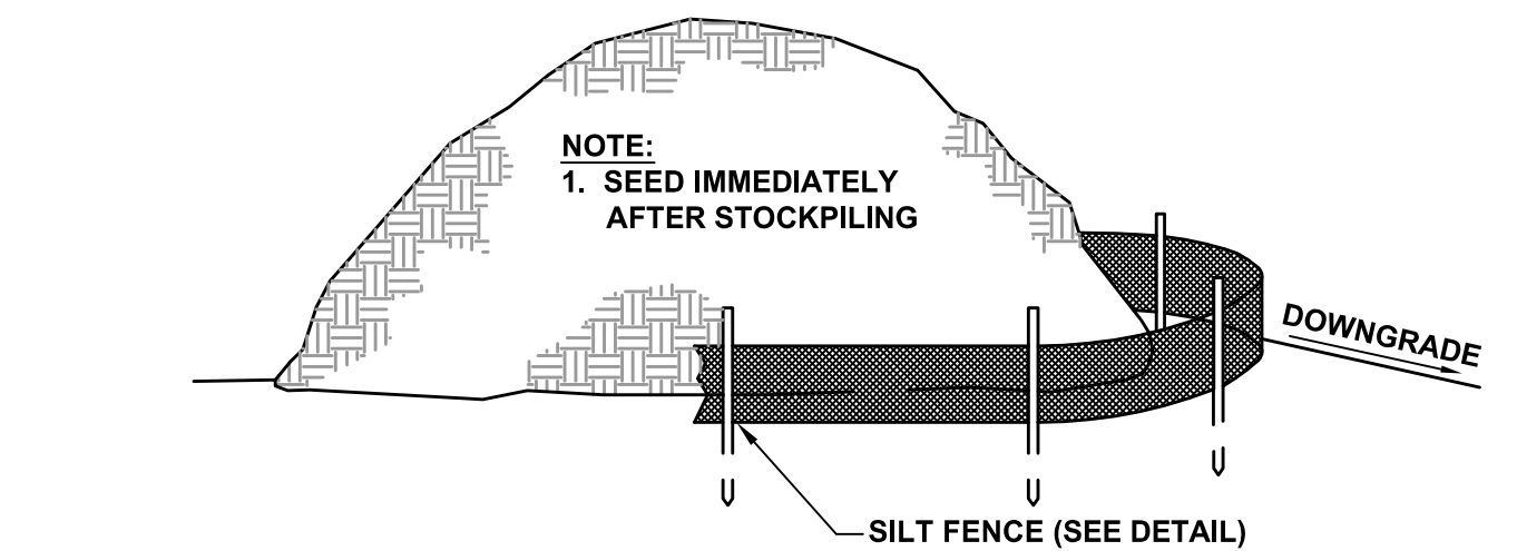
TYPICAL TOPSOIL STOCKPILE N.T.S.
