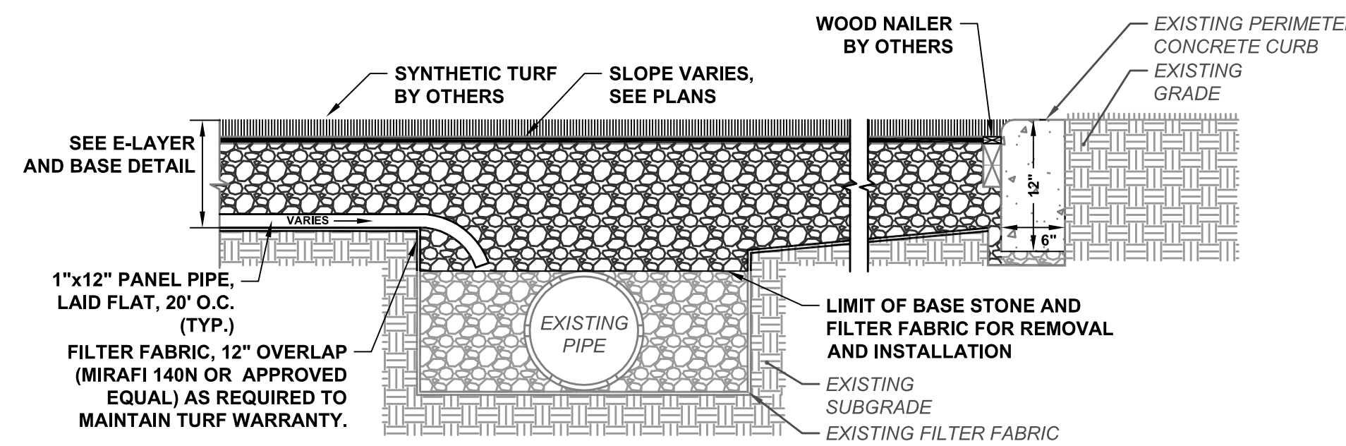
E-LAYER AND BASE TO CONCRETE CURB BY OTHERS N.T.S.
