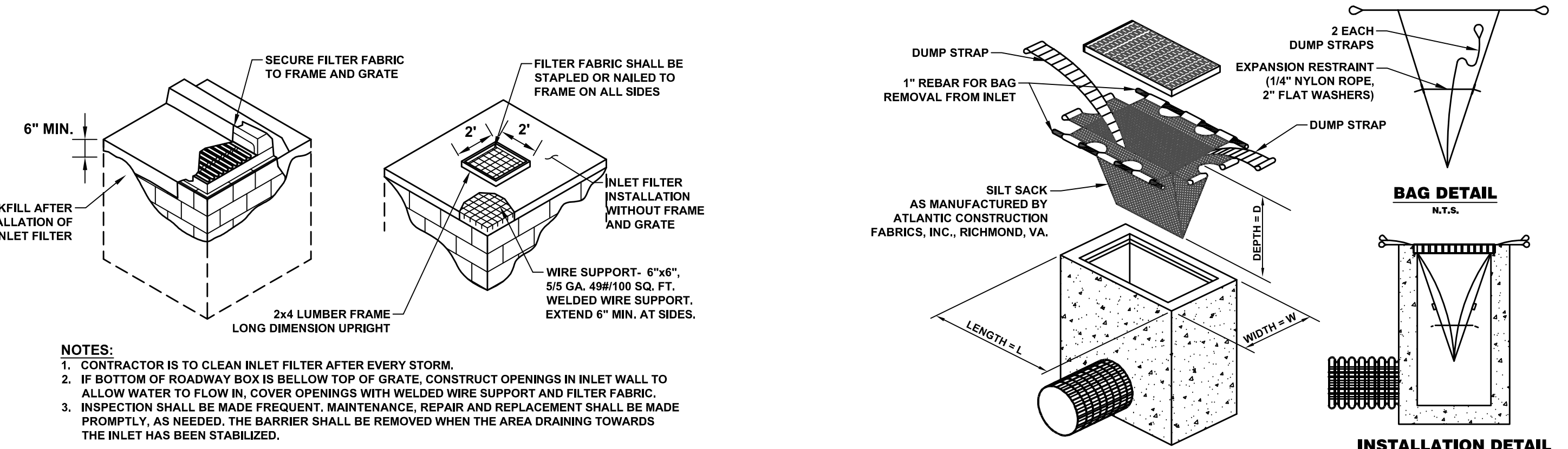
INLET FILTER DETAIL N.T.S.
