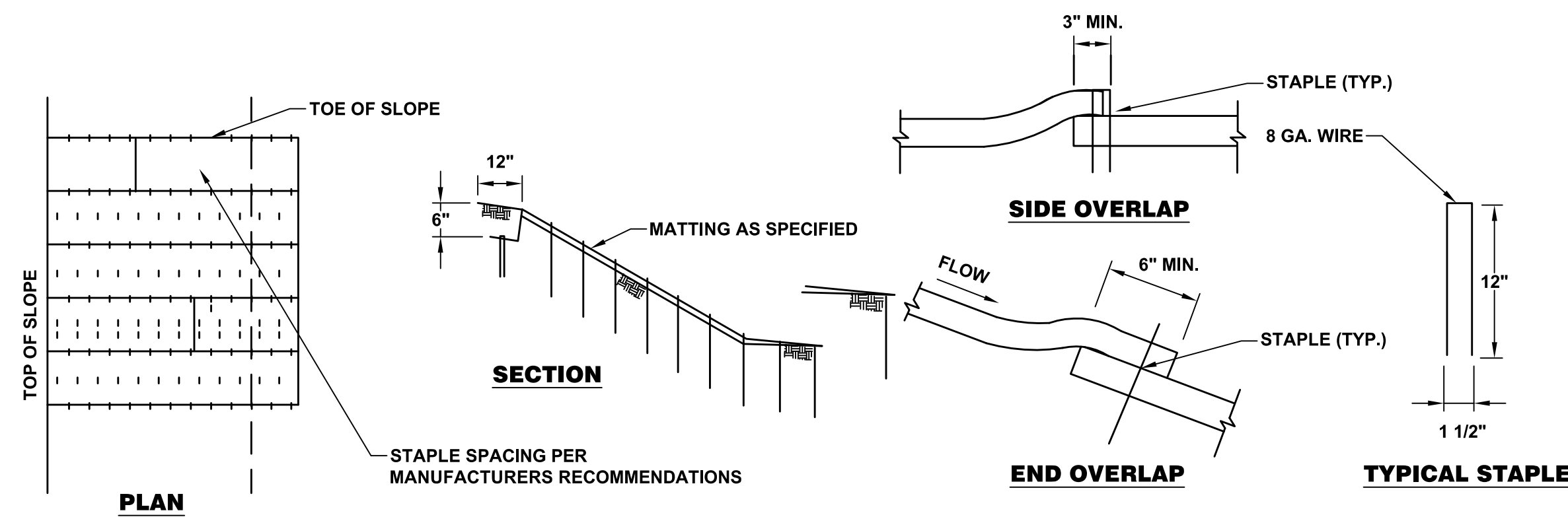
TOPSOIL STOCKPILE STABILIZATION N.T.S.
