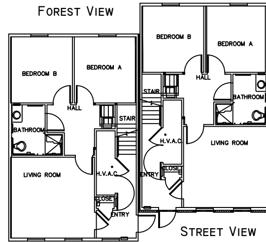
FIRST FLOOR PLAN - TYPE 1
