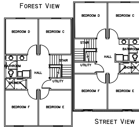
SECOND FLOOR PLAN - TYPE 1
