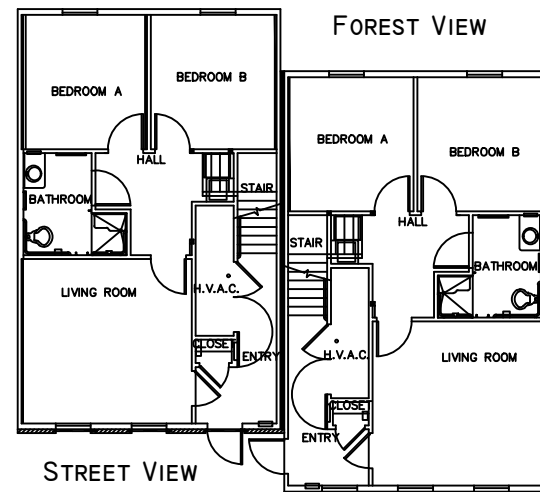
FIRST FLOOR PLAN - TYPE 2
