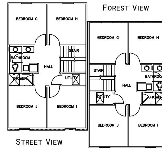
THIRD FLOOR PLAN - TYPE 2
