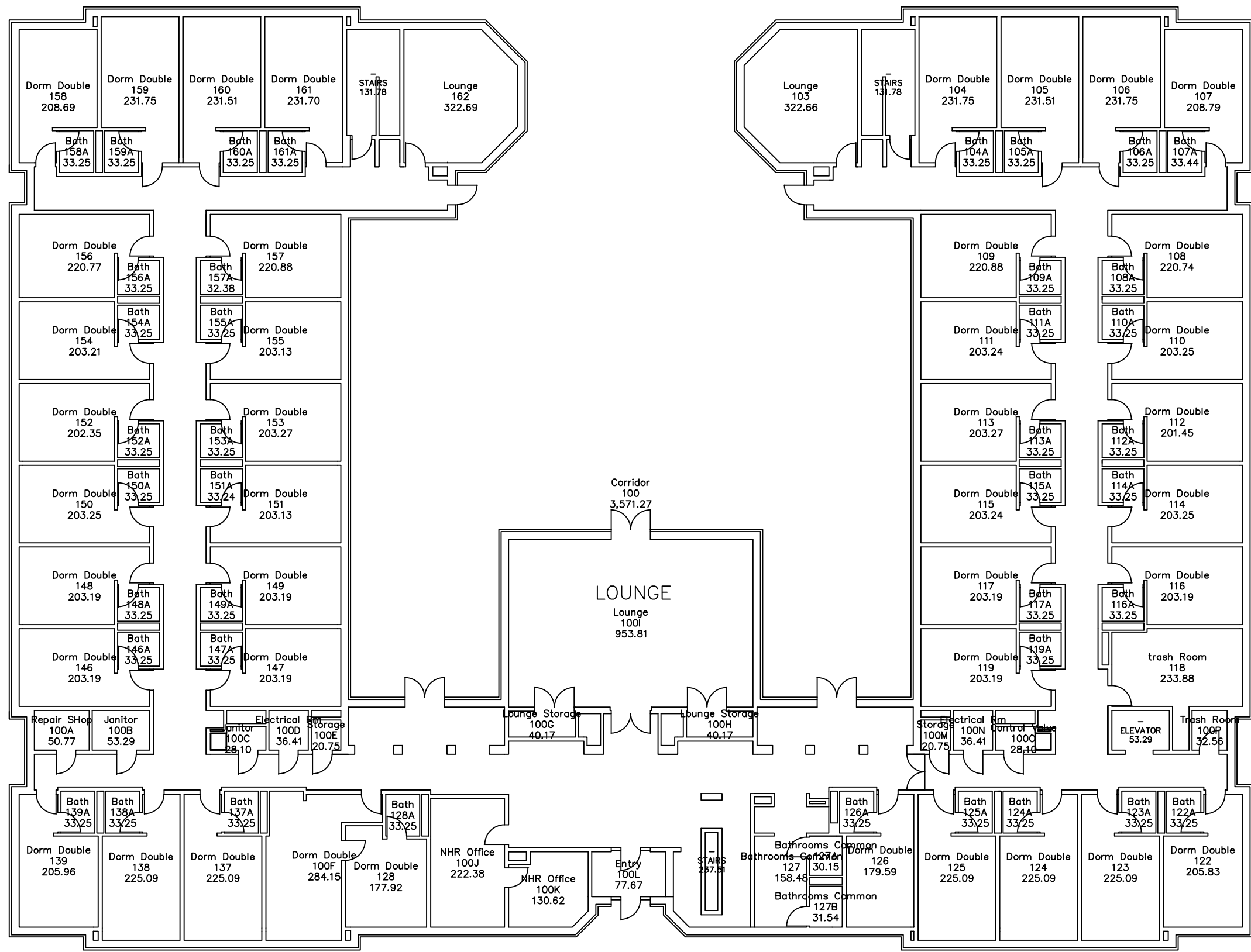
1 FIRST FLOOR PLAN NR.1 SCALE: 1/16" = 1'-0"
