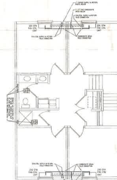
TYPICAL THIRD FLOOR
