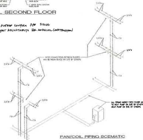
FAN/COIL PIPING SCHEMATIC
