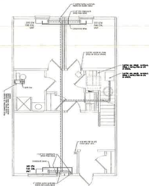
TYPICAL FIRST FLOOR
