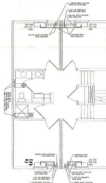
TYPICAL SECOND FLOOR
